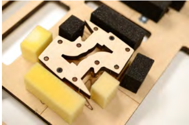
CONVENTIONAL STRIPPER
